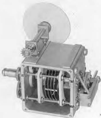
Figure 3. A special type of capacitor used in a precise heterodyne frequency meter. The cast aluminum frame provides both electrical shielding and mechanical stability.
